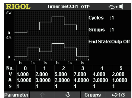
Timing Output Setting
