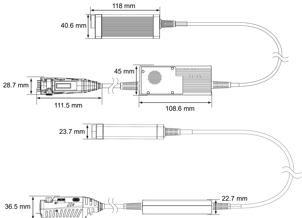
Figure 4.2 Probe Size
