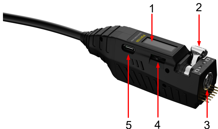
Figure 4.5 Probe Controller
