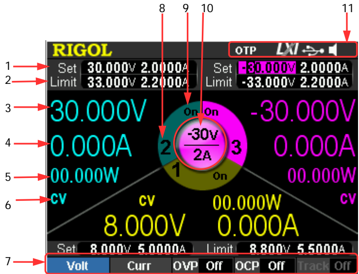
Figure 8 DP831A User Interface
