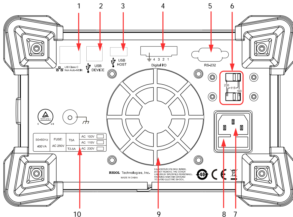
Figure 4 DP831A Rear Panel
