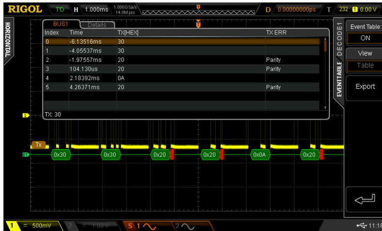
Figure 7-5 RS232 Decoding Table
