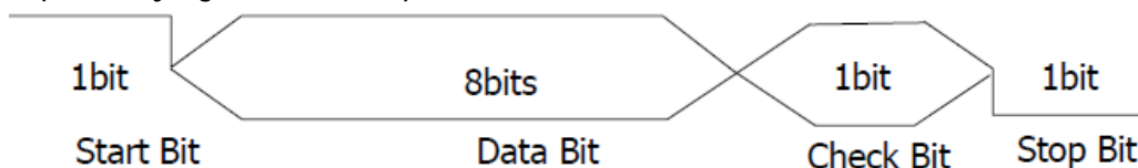
Figure 5-10 RS232 Trigger
