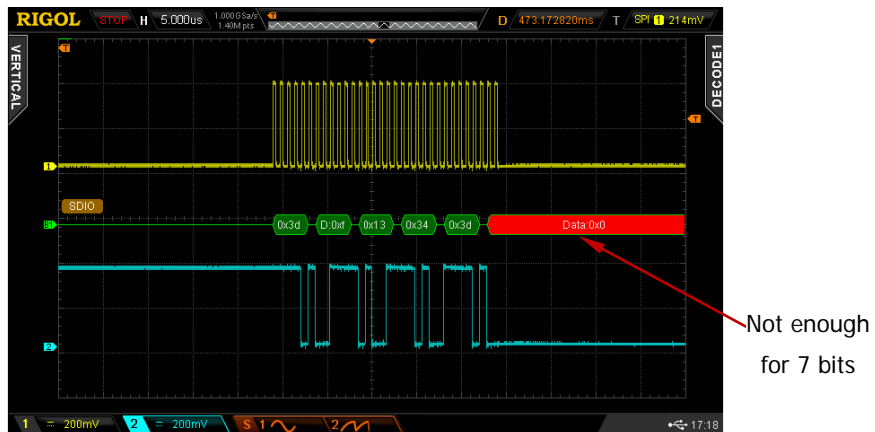
Figure 7-13 Error Expressions During Decoding
