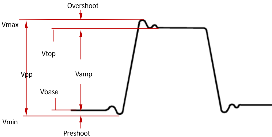
Figure 6-5 Voltage Parameters
