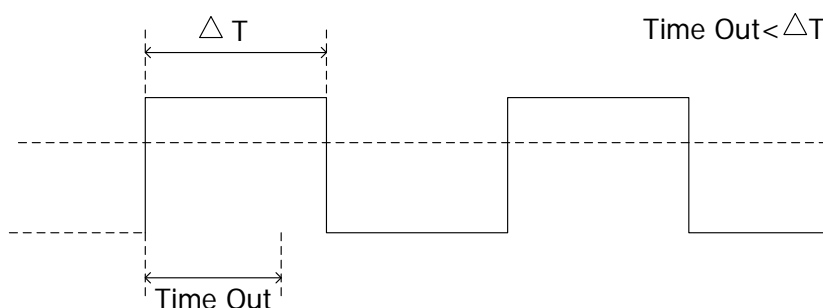
Figure 5-7 TimeOut Trigger
