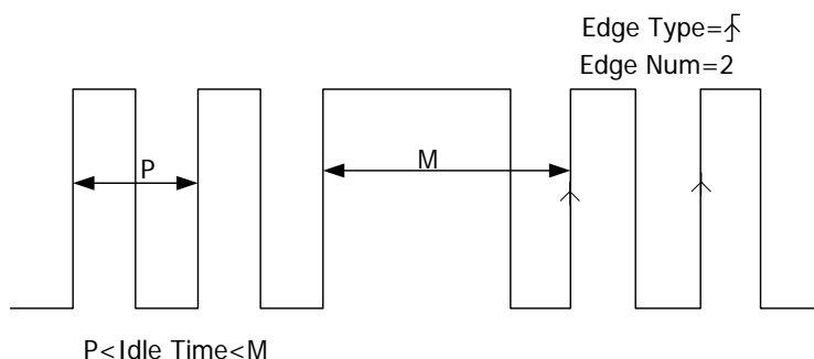
Figure 5-4 Nth Edge Trigger
