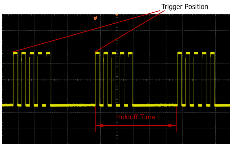
Figure 5-2 Holdoff Time
