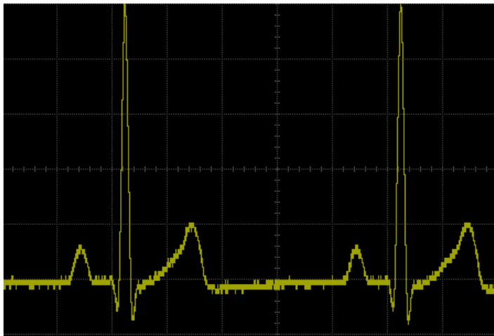
Figure 12-5 Analog ECG
