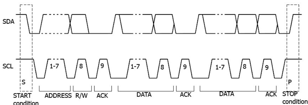
Figure 5-11 I2C Trigger
