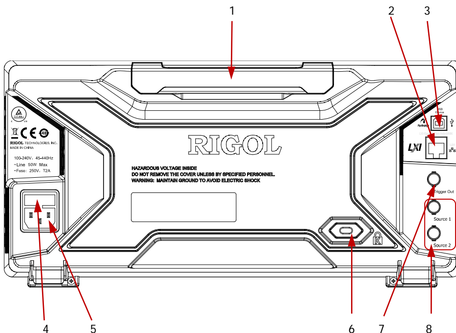
Figure 1-10 Rear Panel Overview
