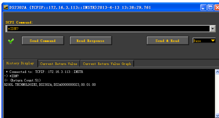
Figure 15-4 Communication Test under Control via LAN
