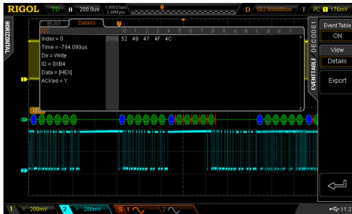
Figure 7-8 I2C Decoding Table (Details)
