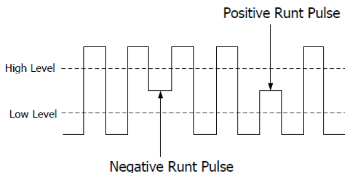
Figure 5-3 Runt Trigger
