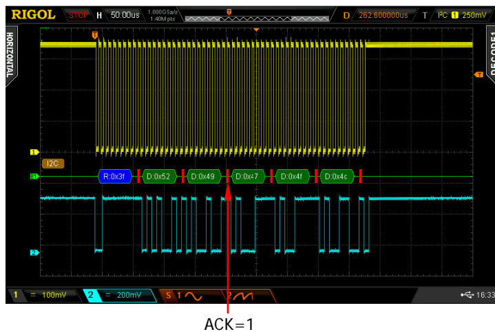
Figure 7-10 Error Expressions during Decoding
