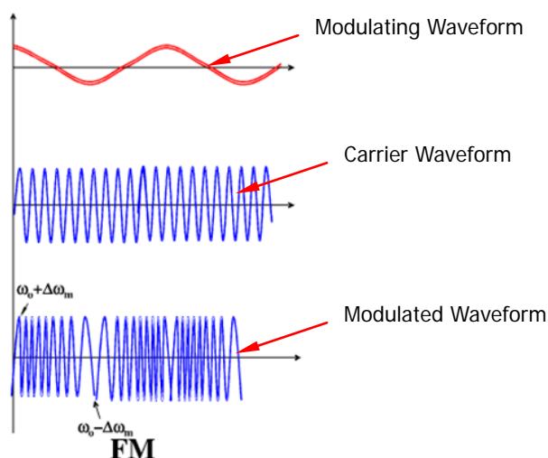
Figure 12-10 FM
