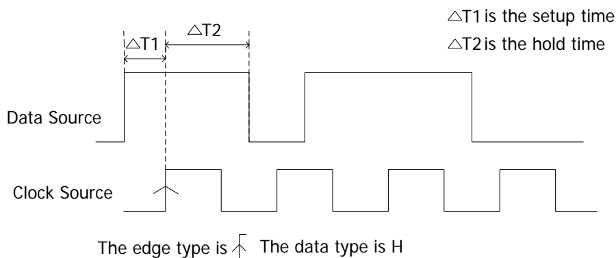
Figure 5-9 Setup/Hold Trigger
