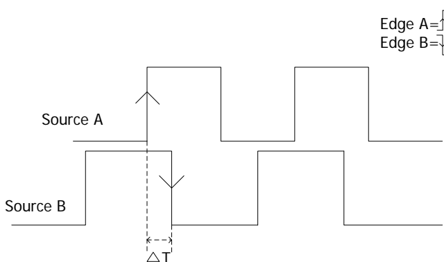
Figure 5-6 Delay Trigger
