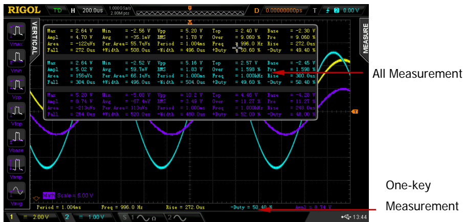
Figure 6-7 All Measurement
