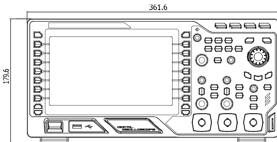
Figure 1-1 Front View
